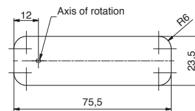
Stamping configuration, glass / steel 0,8–3 mm
