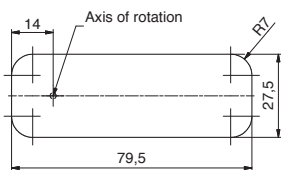
Milling groove, wood / HPL 16–21 mm
